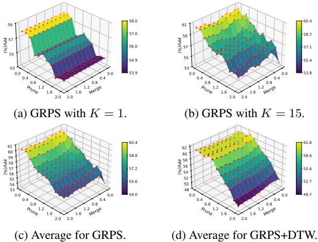
Figure 3: Grid search results.
