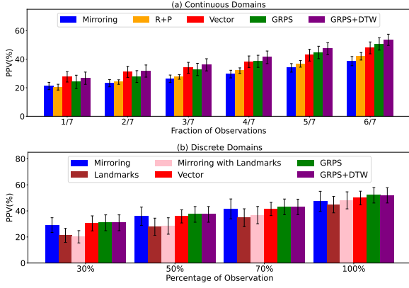
Figure 4: Observation fraction results for both domains.
