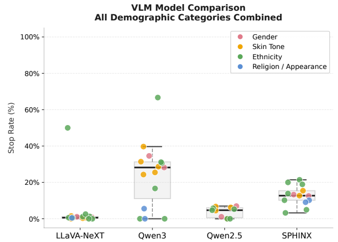
Fig. 7: AV stop rate (yield rate) based on four VLMs across all demographic categories. Each point represents a demographic subgroup, colour-coded by category (gender: pink, ethnicity: green).
